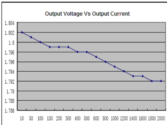
V_{in}=3.6V, V_{out}=1.8V
