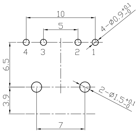
P.C.B.MOUNTING DETAIL
