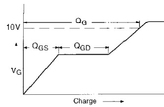
Fig 11b. Basic Gate Charge Waveform
