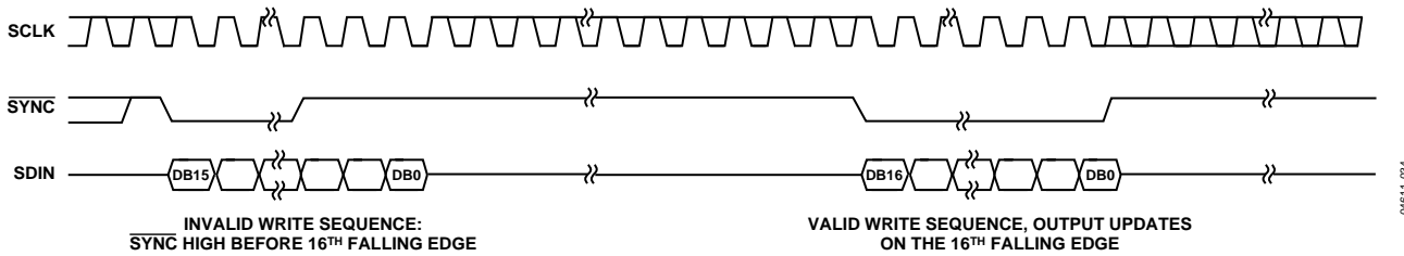
Figure 36. \overline{SYNC} Interrupt Facility
