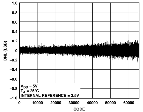
Figure 15. AD5696R DNL
