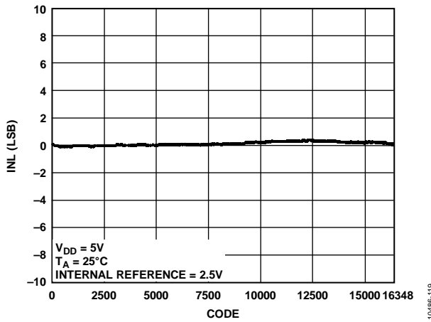
Figure 13. AD5695R INL
