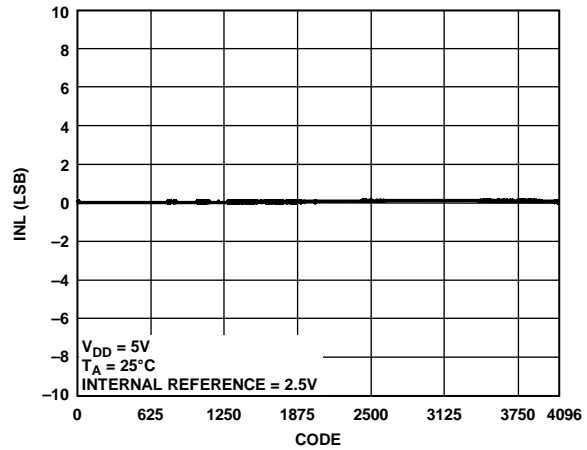
Figure 14. AD5694R INL
