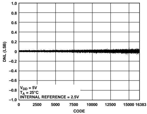
Figure 16. AD5695R DNL
