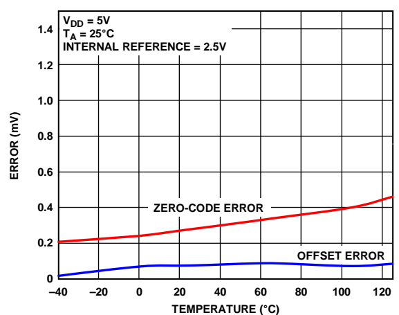
Figure 22. Zero-Code Error and Offset Error vs. Temperature
