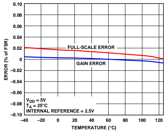
Figure 21. Gain Error and Full-Scale Error vs. Temperature
