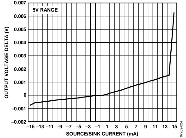
Figure 15. Source and Sink Capability of Output Amplifier
