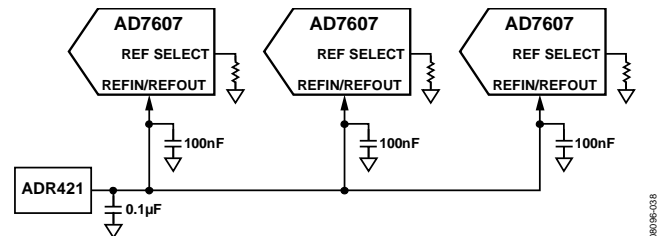
Figure 37. Single External Reference Driving Multiple AD7607 REFIN Pins
