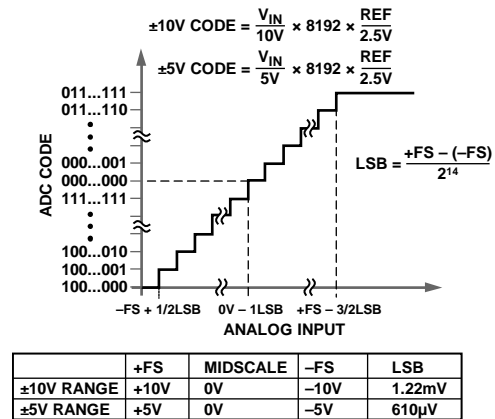
Figure 35. Transfer Characteristics
