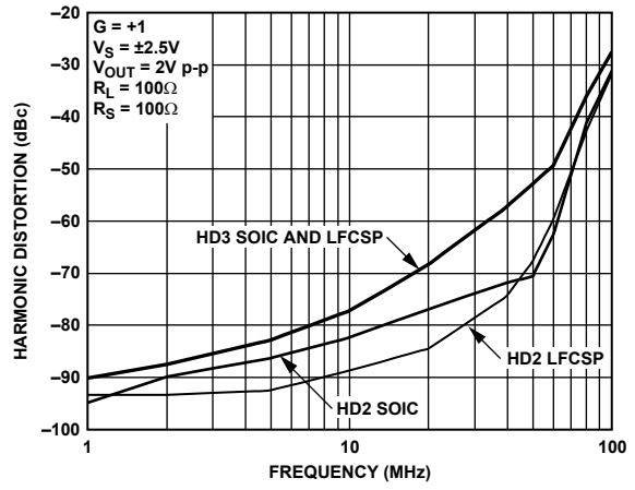
Figure 29. Harmonic Distortion vs. Frequency for Various Packages
