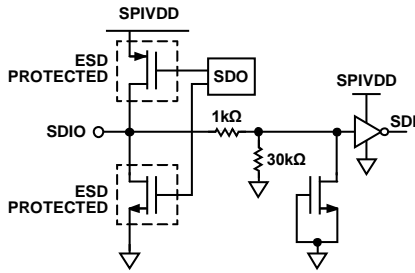
Figure 111. SDIO Input
