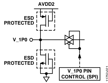
Figure 114. V_1P0 Input/Output
