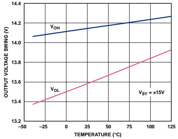
Figure 26. Output Voltage Swing vs. Temperature, V_{SY} = \pm 15V
