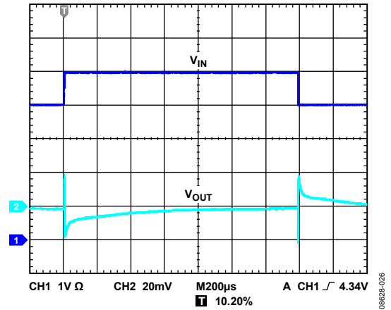
Figure 28. Line Transient Response, V_{IN} = 4V to 5V , C_{IN} = C_{OUT} = 1\mu F , I_{LOAD} = 150mA , CH1 = V_{IN} , CH2 = V_{OUT}
