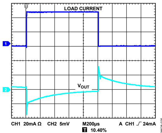
Figure 27. Load Transient Response, C_{IN}, C_{OUT} = 1\mu F , I_{LOAD} = 1mA to 50mA , 200ns Rise Time, CH1 = Load Current, CH2 = V_{OUT}
