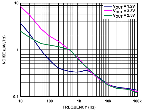
Figure 25. Output Noise Spectral Density, V_{IN} = 5V , I_{LOAD} = 10mA , C_{OUT} = 1\mu F
