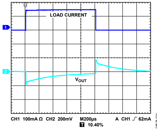
Figure 26. Load Transient Response, C_{IN}, C_{OUT} = 1\mu F , I_{LOAD} = 1mA to 150mA , 200ns Rise Time, CH1 = Load Current, CH2 = V_{OUT}
