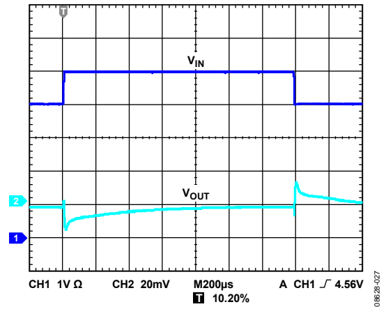
Figure 29. Line Transient Response, V_{IN} = 4V to 5V , C_{IN} = 1\mu F , C_{OUT} = 10\mu F , I_{LOAD} = 150mA , CH1 = V_{IN} , CH2 = V_{OUT}
