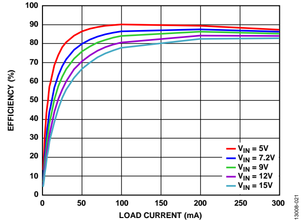
Figure 21. Channel 2 PWM Efficiency vs. Load Current, V_{OUT2} = 2.5\text{ V}
