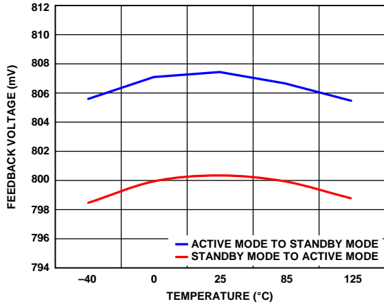
Figure 28. Channel 2 Feedback Voltage of Hysteresis Mode vs. Temperature
