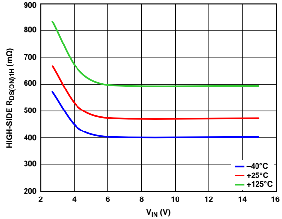
Figure 31. Channel 1 High-Side R_{DS(ON)1H} vs. V_{IN}
