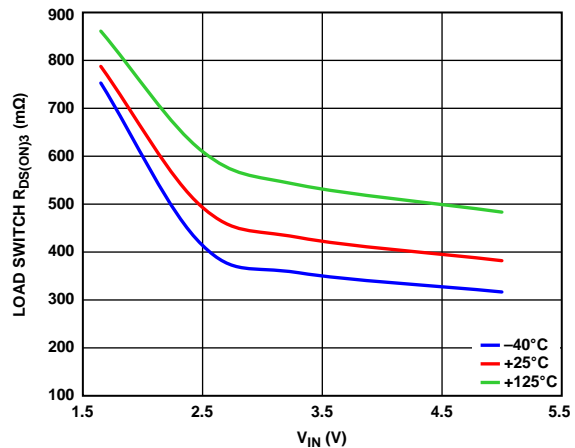
Figure 33. Channel 3 Load Switch R_{DS(ON)3} vs. V_{IN}
