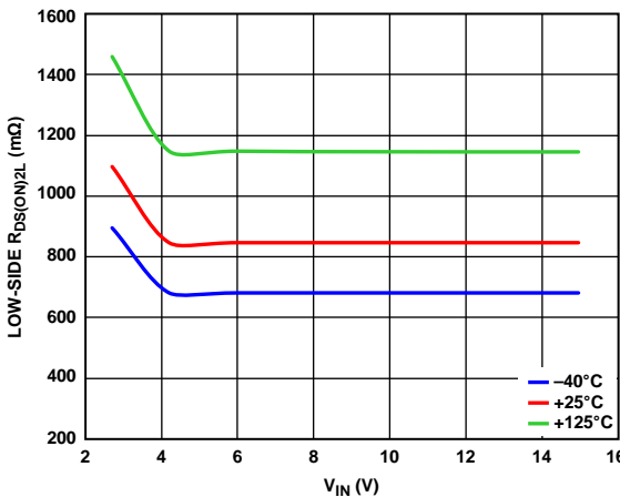
Figure 30. Channel 2 Low-Side R_{DS(ON)2L} vs. V_{IN}
