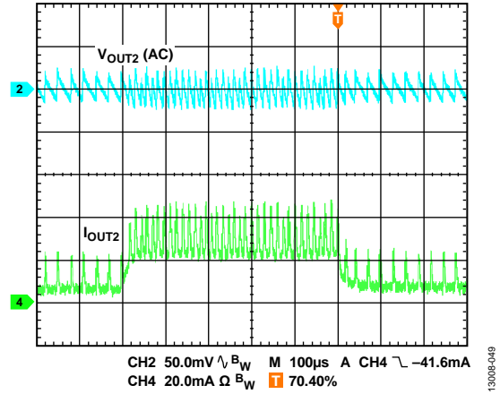
Figure 49. Channel 2 Hysteresis Mode Load Transient (10 mA to 30 mA Load Step)
