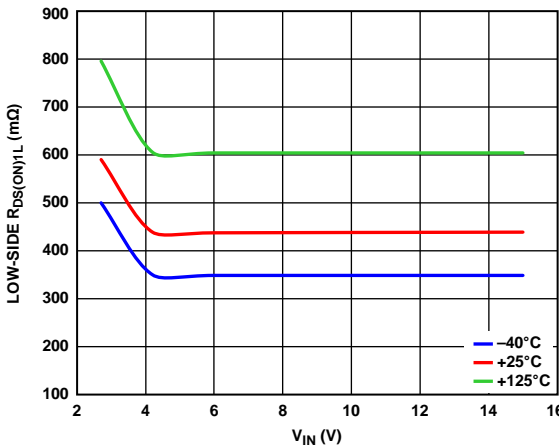
Figure 29. Channel 1 Low-Side R_{DS(ON)1L} vs. V_{IN}
