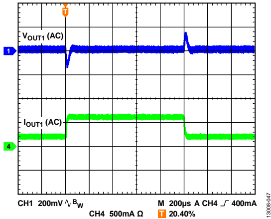
Figure 47. Channel 1 Load Transient (0.2 A to 0.6 A Load Step)
