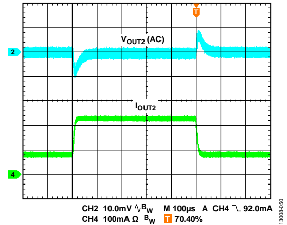
Figure 50. Channel 2 PWM Mode Load Transient (75 mA to 225 mA Load Step)
