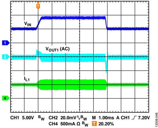
Figure 46. Channel 1 Line Transient in PWM Mode
