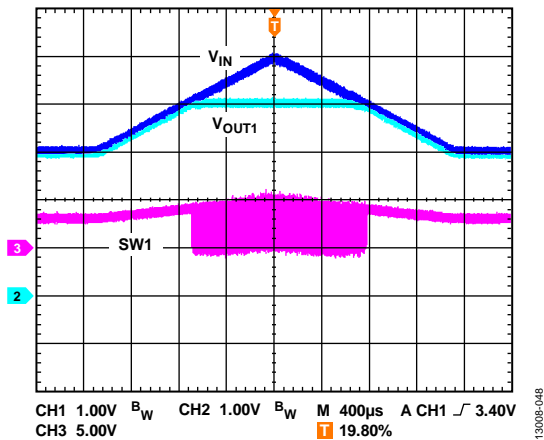
Figure 48. Channel 1 100% Duty Operation in PWM Mode
