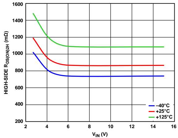
Figure 32. Channel 2 High-Side R_{DS(ON)2H} vs. V_{IN}
