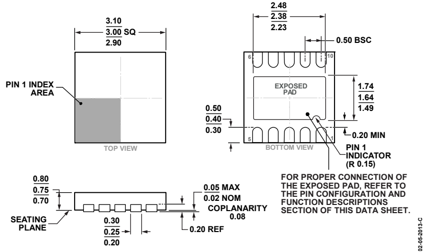
Figure 64. 10-Lead Lead Frame Chip Scale Package [LFCSP] 3 mm x 3 mm Body and 0.75 mm Package Height (CP-10-9) Dimensions shown in millimeters
