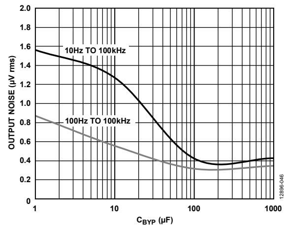
Figure 44. RMS Noise vs. Bypass Capacitance ( C_{BYP} )
