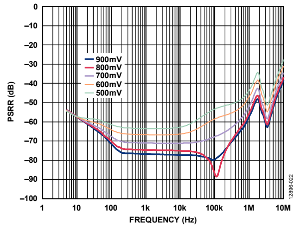
Figure 22. Power Supply Rejection Ratio (PSRR) vs. Frequency at Various Headroom Voltages, V_{OUT} = 3.3 V , 2 A Load
