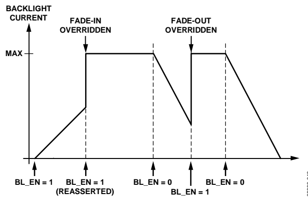
Figure 39. Fade Override Function (FOVR Is High)
