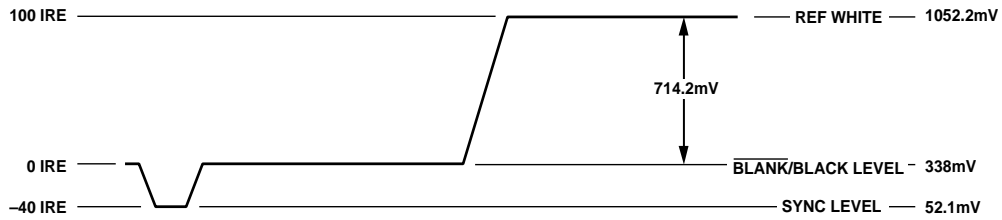
Figure 66. NTSC Luma Video Levels
