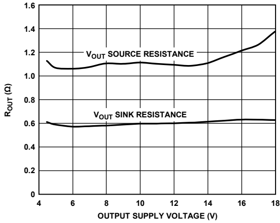
Figure 17. Typical Output Resistance vs. Output Supply Voltage
