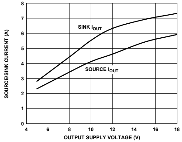
Figure 18. Typical Output Current vs. Output Supply Voltage
