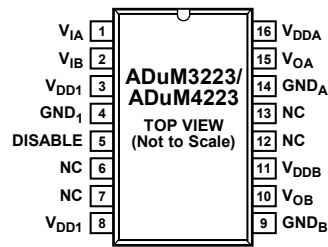
Figure 4. Pin Configuration
