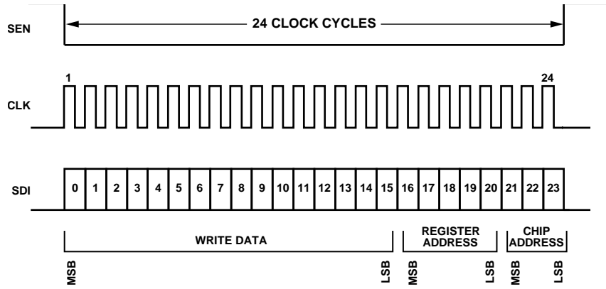
Figure 50. Timing Diagram, SPI Register Write
