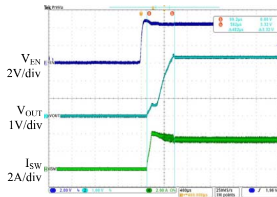
Time 400µs/div
