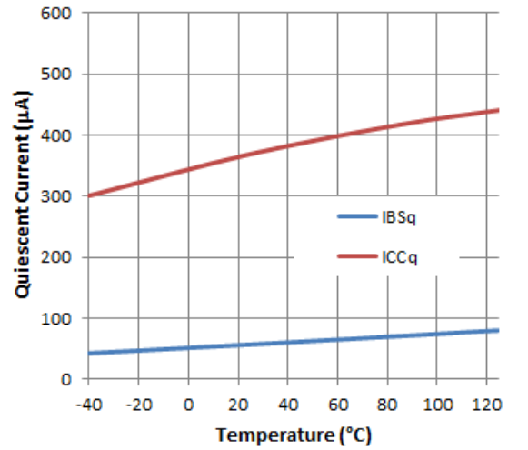
Figure 13. Quiescent Current vs. Temperature
