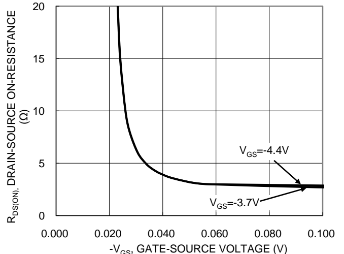
Figure 4. Typical On-Resistance vs. Gate Voltage
