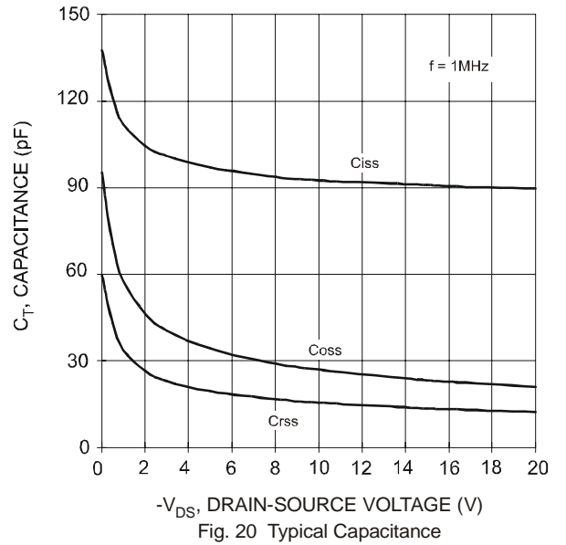
Fig. 20 Typical Capacitance
