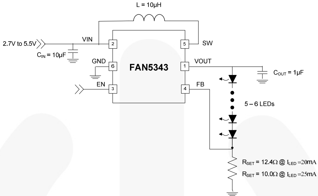
Figure 1. Typical Application
