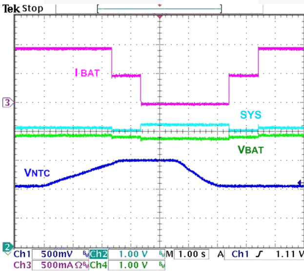
Figure 21. Charging vs. Temperature (NTC), +30^\circ\text{C} to -10^\circ\text{C} 3.7\text{ V}_{BAT} , I_{CHRG}=950\text{ mA} , No I_{BUSLIM} , 100\ \Omega\text{ SYS Load}
