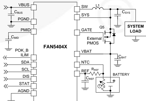
Figure 1. Typical Application
