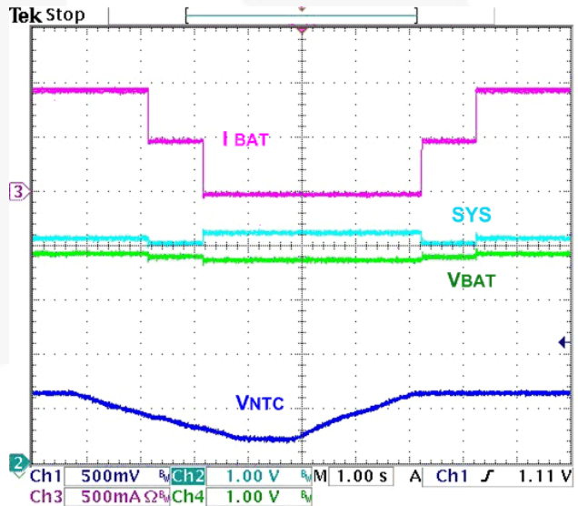
Figure 22. Charging vs. Temperature (NTC), +30^\circ\text{C} to +70^\circ\text{C} 3.7\text{ V}_{BAT} , I_{CHRG}=950\text{ mA} , No I_{BUSLIM} , 100\ \Omega\text{ SYS Load}
