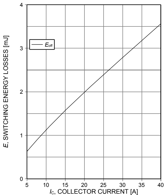
Figure 12. Typical switching energy losses as a function of collector current (inductive load, T_{vj}=175^\circ\text{C} , V_{CE}=600\text{V} , V_{GE}=0/15\text{V} , R_{G(on)}=10\Omega , R_{G(off)}=10\Omega , dynamic test circuit in Figure E)
