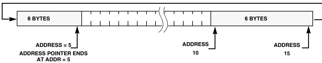
FIGURE 18. WRITING 12 BYTES TO A 16-BYTE MEMORY PAGE STARTING AT ADDRESS 10
