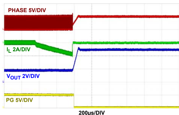
FIGURE 40. OVERTOVOLTAGE PROTECTION (ISL80030A) f_{SW} = 2\text{MHz} , V_{IN} = 5\text{V} , PWM, T_A = +25^\circ\text{C}
