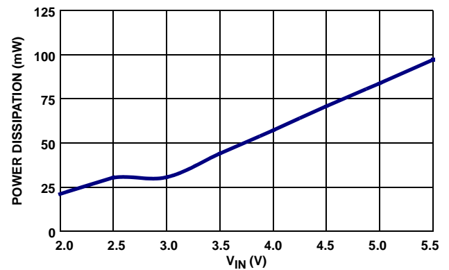
FIGURE 6. POWER DISSIPATION WITH NO LOAD vs V IN (PWM V OUT = 1.8V)
