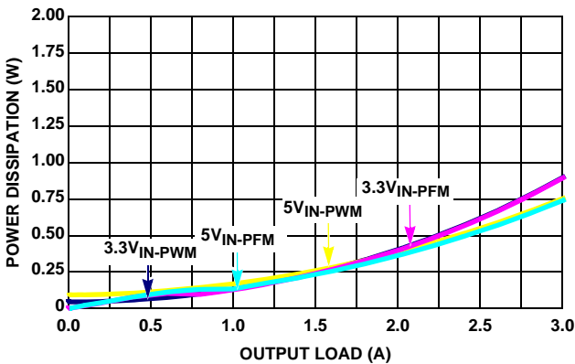
FIGURE 5. POWER DISSIPATION vs LOAD (1MHz, V OUT = 1.8V)
