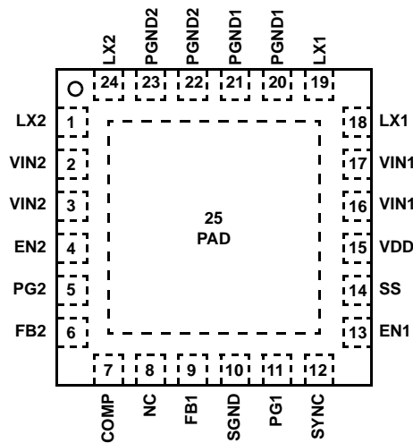
ISL8036, ISL8036A (24 LD QFN) TOP VIEW
