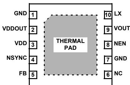
ISL97701 (10 LD 3X3 DFN) TOP VIEW
