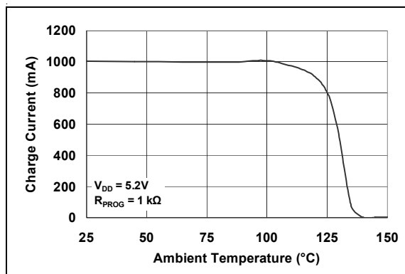
FIGURE 4-3: Thermal Regulation
