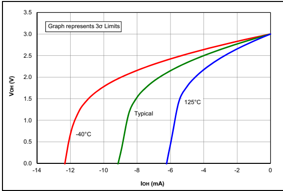
FIGURE 36-47: V_{OH} vs. I_{OH} Over Temperature, V_{DD} = 3.0V .
