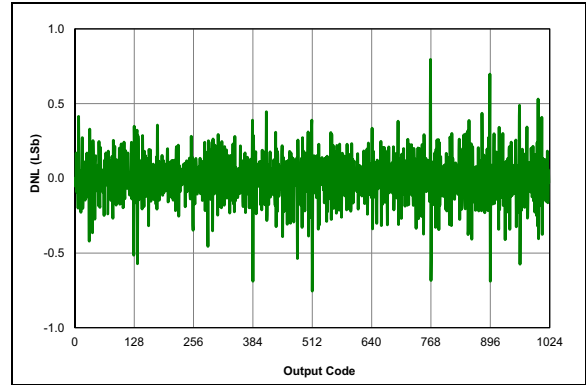
FIGURE 36-71: ADC 10-bit Mode, Single-Ended DNL, V_{DD} = 3.0V , T_{AD} = 1\ \mu\text{S} , 25^\circ\text{C} .
