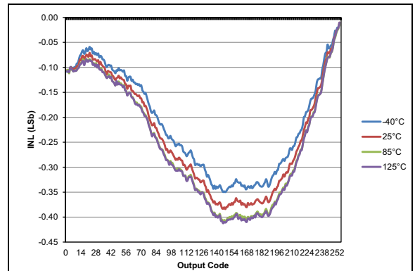
FIGURE 36-101: Typical DAC INL Error, V_{DD} = 5.0V , V_{REF} = \text{External } 5V , PIC16F1615/9 Only.
