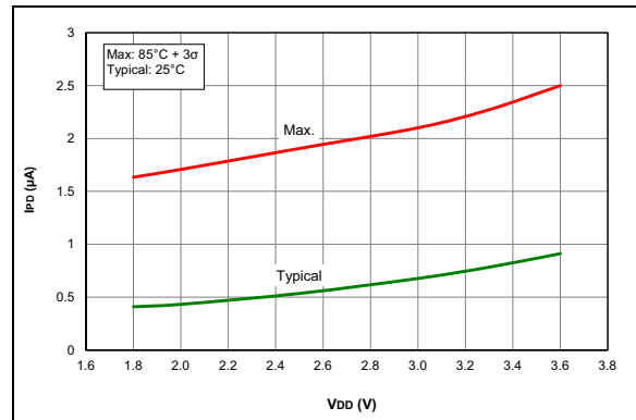
FIGURE 36-29: I_{PD} , Watchdog Timer (WDT), PIC16LF1615/9 Only.
