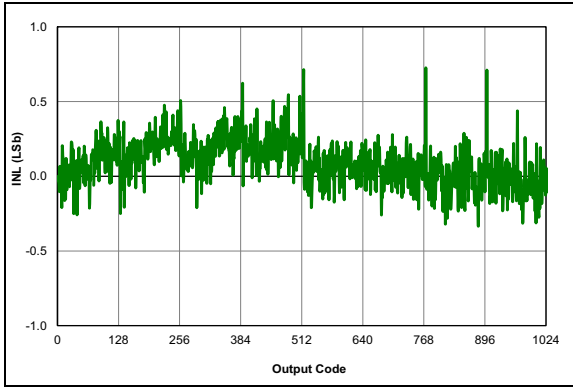
FIGURE 36-73: ADC 10-bit Mode, Single-Ended INL, V_{DD} = 3.0V , T_{AD} = 1\ \mu\text{S} , 25^\circ\text{C} .
