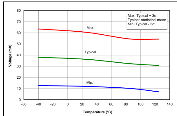
FIGURE 36-60: Brown-Out Reset Hysteresis, High Trip Point ( BORV = 0 ).
