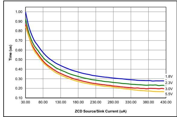
FIGURE 36-110: ZCD Pin Response Time over Current, Typical Measured Values from -40^\circ\text{C} to 125^\circ\text{C} .
