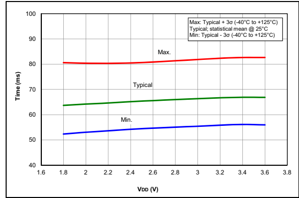
FIGURE 36-64: PWRT Period, PIC16LF1615/9 Only.
