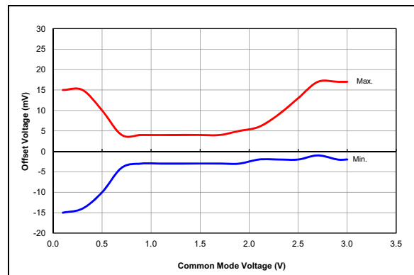
FIGURE 36-89: Comparator Offset, NP Mode ( CxSP = 1 ), V_{DD} = 3.0V , Typical Measured Values at 25^\circ\text{C} .
