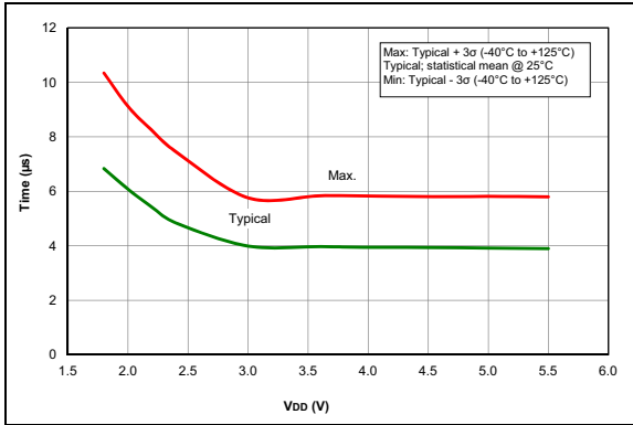
FIGURE 36-68: Wake From Sleep, V_{REGPM} = 0 .
