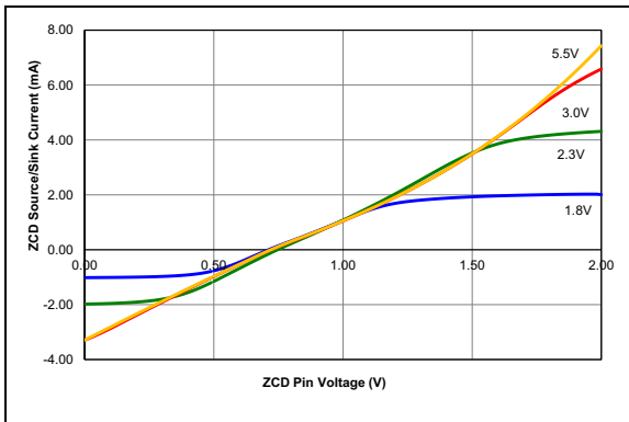
FIGURE 36-109: ZCD Pin Current over ZCD Pin Voltage, Typical Measured Values from -40^\circ\text{C} to 125^\circ\text{C} .
