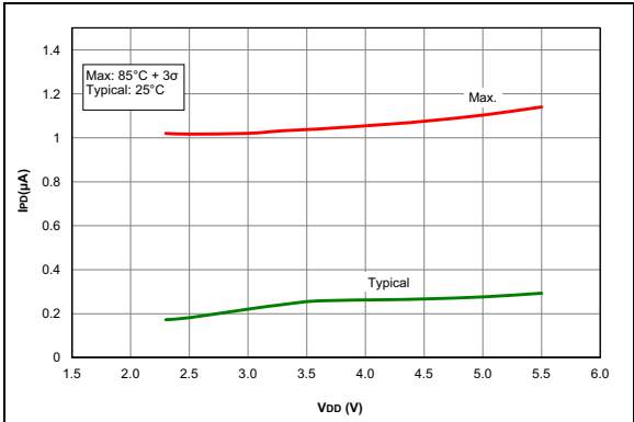
FIGURE 36-40: I_{PD} , ADC Non-Converting, PIC16F1615/9 Only.
