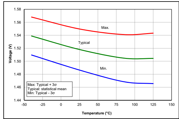
FIGURE 36-66: POR Rearm Voltage, NP Mode ( V_{REGPM1} = 0 ), PIC16F1615/9 Only.
