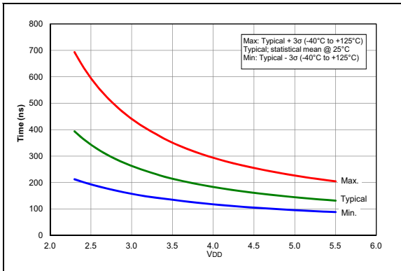
FIGURE 36-97: Comparator Output Filter Delay Time Over Temp., NP Mode ( CxSP = 1 ), Typical Measured Values, PIC16F1615/9 Only.
