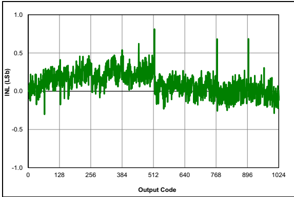
FIGURE 36-74: ADC 10-bit Mode, Single-Ended INL, V_{DD} = 3.0V , T_{AD} = 4\ \mu\text{S} , 25^\circ\text{C} .
