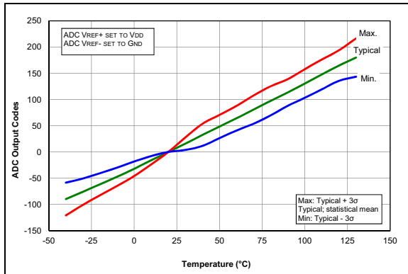
FIGURE 36-85: Temp. Indicator Slope Normalized to 20^\circ\text{C} , Low Range, V_{DD} = 1.8V , PIC16LF1615/9 Only.
