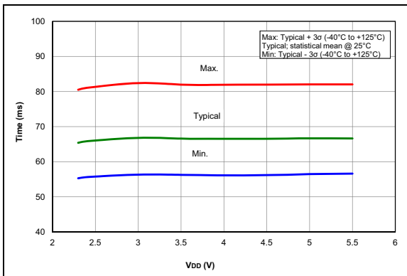
FIGURE 36-63: PWRT Period, PIC16F1615/9 Only.
