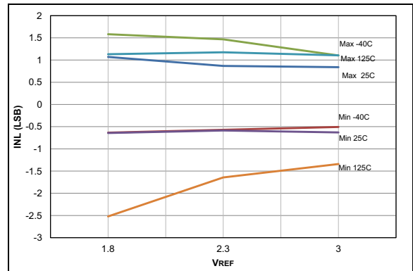
FIGURE 36-78: ADC 10-bit Mode, Single-Ended INL, V_{DD} = 3.0V , T_{AD} = 1\ \mu\text{S} .
