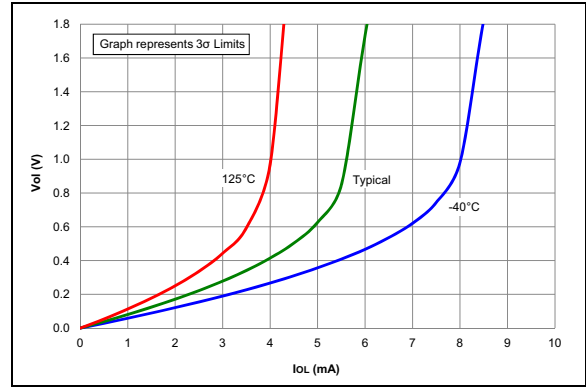
FIGURE 36-50: V_{OL} vs. I_{OL} Over Temperature, V_{DD} = 1.8V , PIC16LF1615/9 Only.
