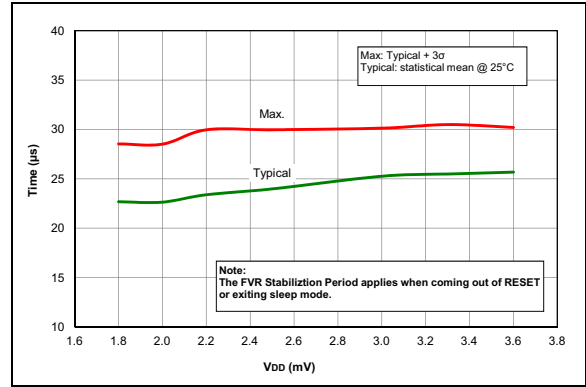
FIGURE 36-70: FVR Stabilization Period, PIC16LF1615/9 Only.
