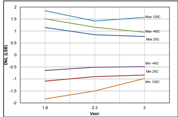
FIGURE 36-77: ADC 10-bit Mode, Single-Ended DNL, V_{DD} = 3.0V , T_{AD} = 1\ \mu\text{S} .
