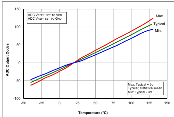
FIGURE 36-86: Temp. Indicator Slope Normalized to 20^\circ\text{C} , Low Range, V_{DD} = 3.0V , PIC16LF1615/9 Only.
