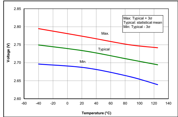
FIGURE 36-59: Brown-Out Reset Voltage, High Trip Point ( BORV = 0 ).
