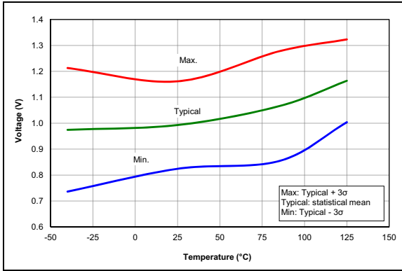
FIGURE 36-67: POR Rearm Voltage, NP Mode, PIC16LF1615/9 Only.
