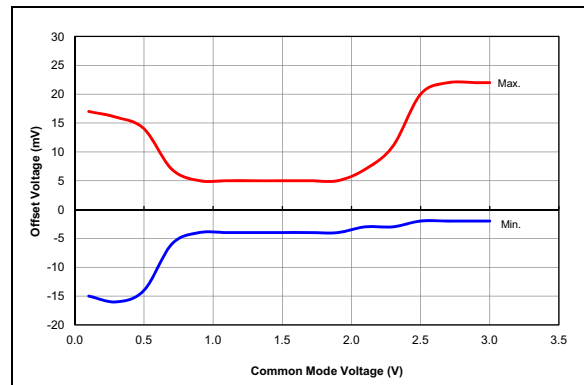
FIGURE 36-90: Comparator Offset, NP Mode ( CxSP = 1 ), V_{DD} = 3.0V , Typical Measured Values From -40^\circ\text{C} to 125^\circ\text{C} .
