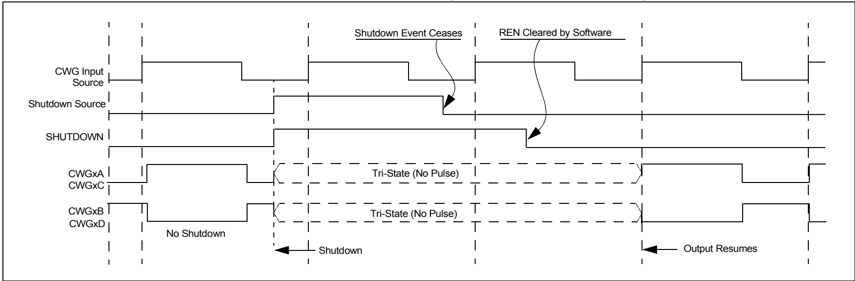
FIGURE 28-14: SHUTDOWN FUNCTIONALITY, AUTO-RESTART ENABLED (REN = 1, LSAC = 01, LSB0 = 01)
