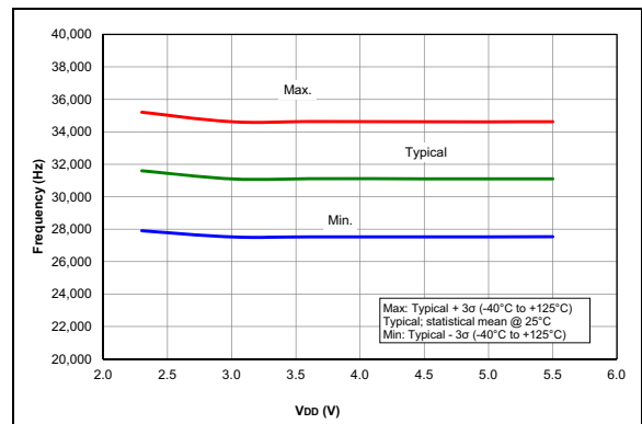
FIGURE 36-52: LFINTOSC Frequency, PIC16F1615/9 Only.
