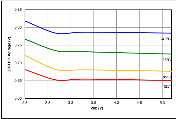
FIGURE 36-107: ZCD Pin Voltage, Typical Measured Values.
