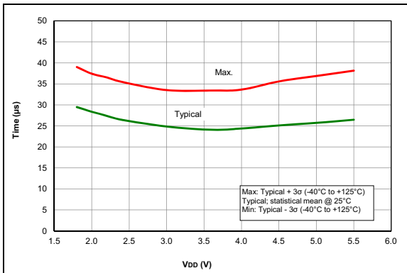
FIGURE 36-69: Wake From Sleep, V_{REGPM} = 1 .
