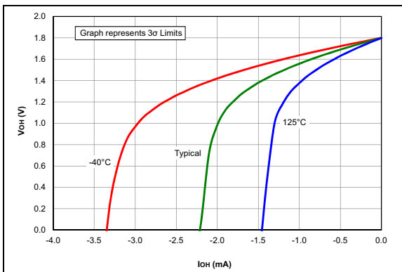
FIGURE 36-49: V_{OH} vs. I_{OH} Over Temperature, V_{DD} = 1.8V , PIC16LF1615/9 Only.
