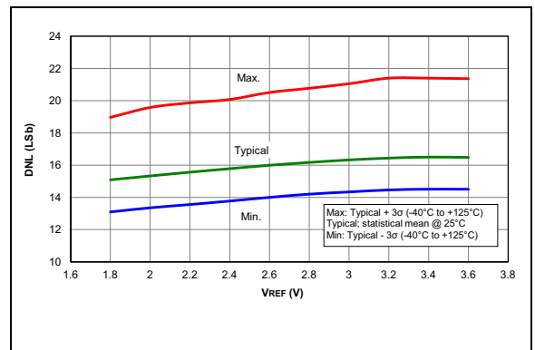
FIGURE 36-102: DAC INL Error, V_{DD} = 3.0V .
