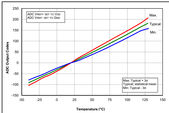
FIGURE 36-87: Temp. Indicator Slope Normalized to 20^\circ\text{C} , High Range, V_{DD} = 3.6V , PIC16LF1615/9 Only.
