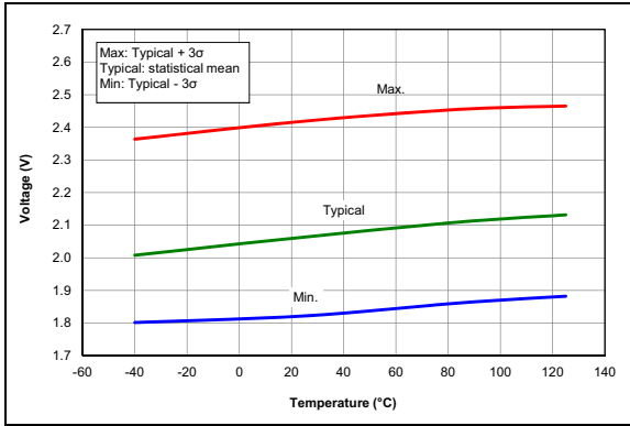
FIGURE 36-61: LPBOR Reset Voltage.
