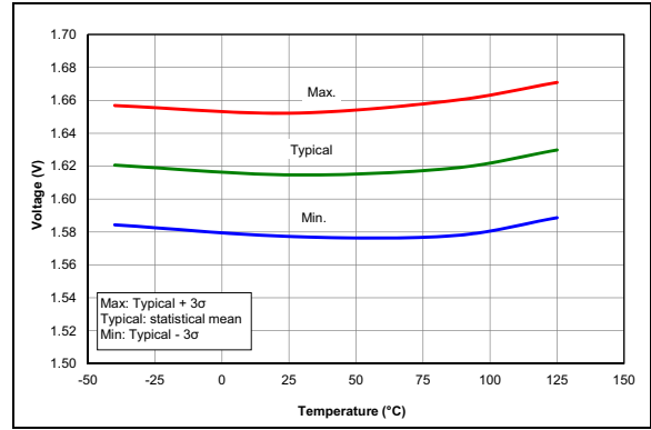
FIGURE 36-65: POR Release Voltage.
