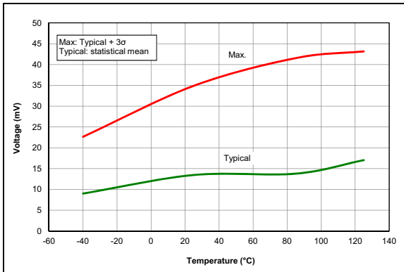
FIGURE 36-62: LPBOR Reset Hysteresis.
