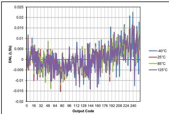
FIGURE 36-98: Typical DAC DNL Error, V_{DD} = 3.0V , V_{REF} = \text{External } 3V .
