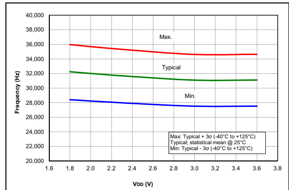
FIGURE 36-51: LFINTOSC Frequency, PIC16LF1615/9 Only.
