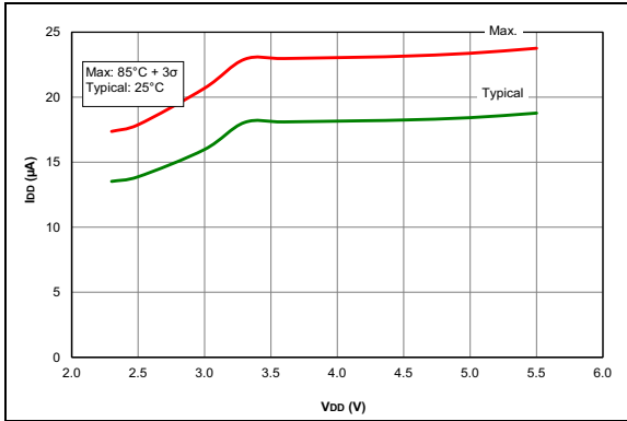
FIGURE 36-108: ZCD Response Time over Voltage Typical Measured Values.
