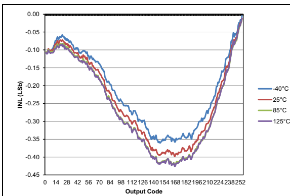
FIGURE 36-99: Typical DAC INL Error, V_{DD} = 3.0V , V_{REF} = \text{External } 3V .
