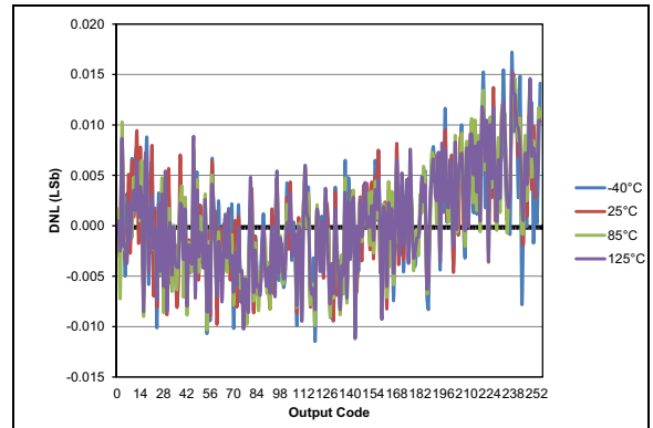
FIGURE 36-100: Typical DAC INL Error, V_{DD} = 5.0V , V_{REF} = \text{External } 5V , PIC16F1615/9 Only.
