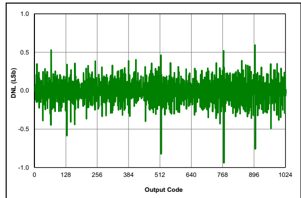
FIGURE 36-72: ADC 10-bit Mode, Single-Ended DNL, V_{DD} = 3.0V , T_{AD} = 4\ \mu\text{S} , 25^\circ\text{C} .
