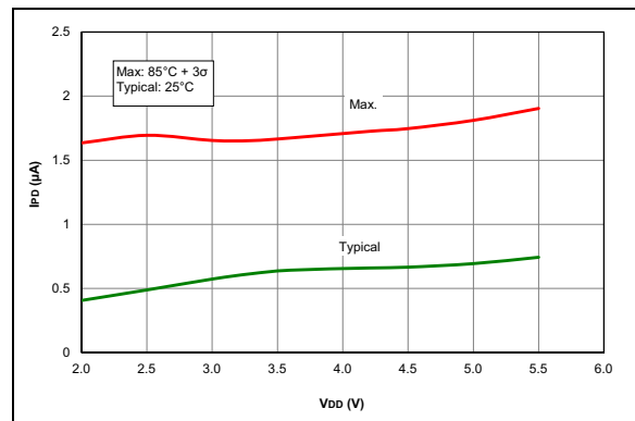
FIGURE 36-30: I_{PD} , Watchdog Timer (WDT), PIC16F1615/9 Only.
