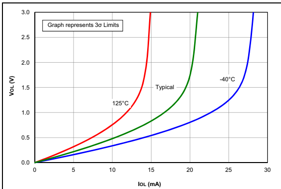
FIGURE 36-48: V_{OL} vs. I_{OL} Over Temperature, V_{DD} = 3.0V .
