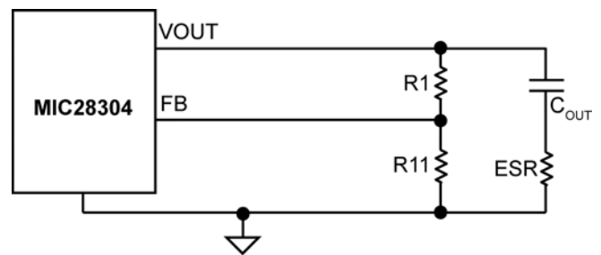
Figure 9. Enough Ripple at FB
