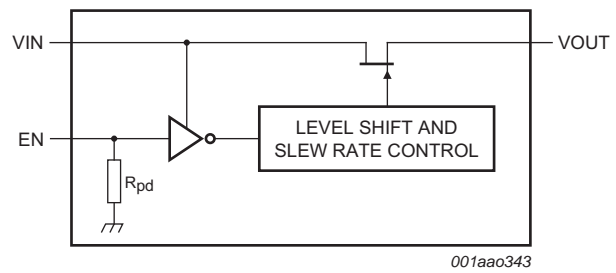
Fig 2. Logic diagram (simplified schematic)
