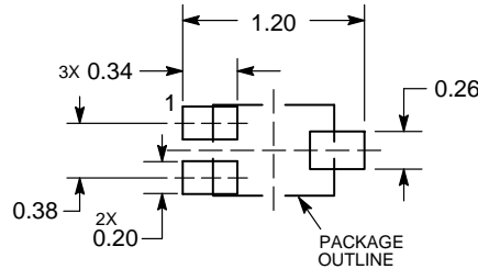
SOLDERING FOOTPRINT*
