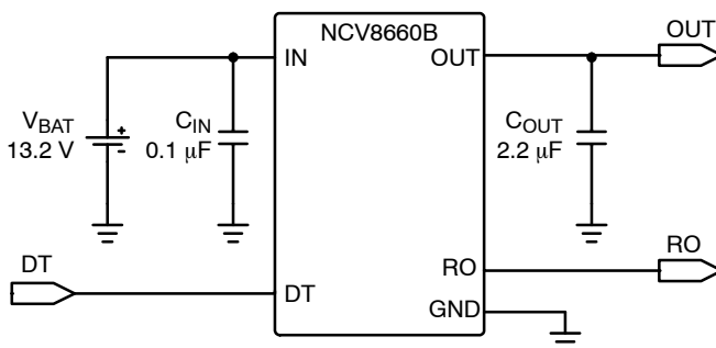
Figure 1. Application Diagram
