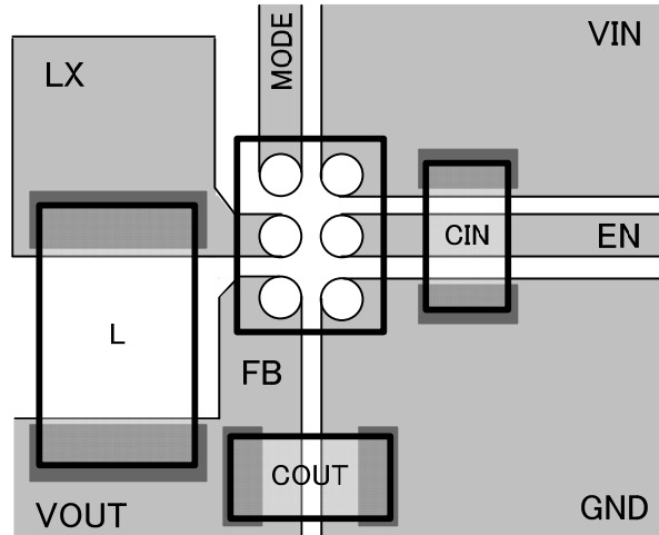
Figure 16. PCB layout
