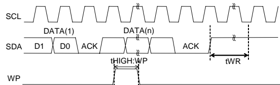
Figure 1-(e) WP timing at write cancel
