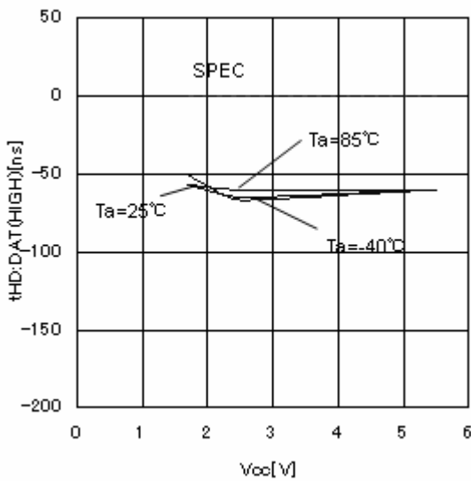
Figure 16. Input data hold time tHD:DAT
