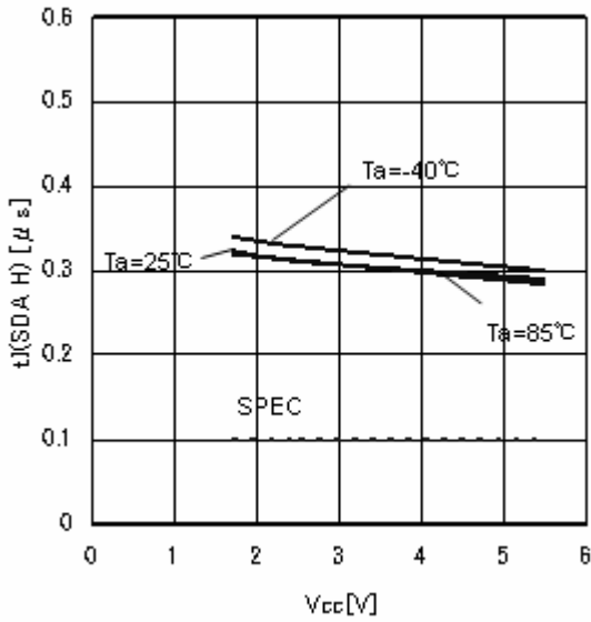
Figure 26. Noise removal time t_l (SDA H)
