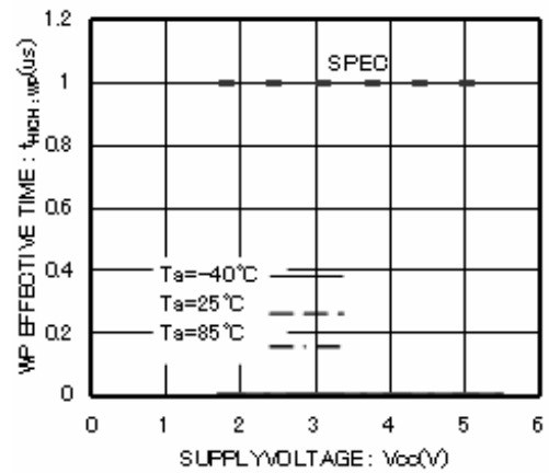
Figure 29. WP effective time t_{\text{HIGH:WP}}
