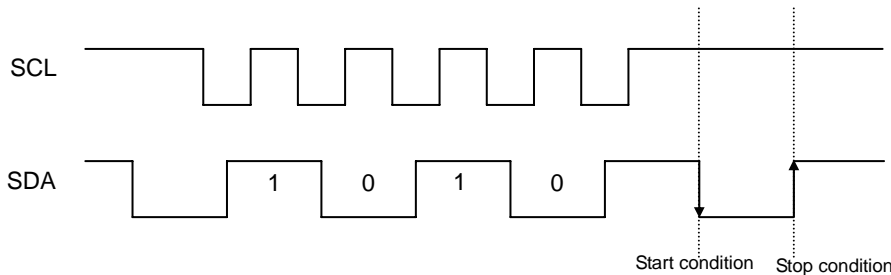
Figure 40. Case of cancel by start, stop condition during slave address input
