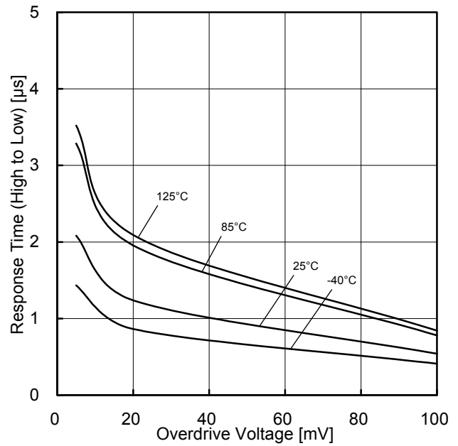
Figure 23. Response Time (High to Low) vs Overdrive Voltage ( V_{CC^+}=5V , V_{RL}=5V , R_L=5.1k\Omega )
