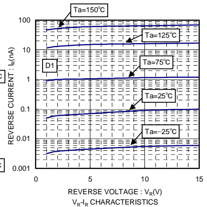
V_R - I_R CHARACTERISTICS
