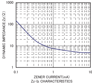
Zz-Iz CHARACTERISTICS
