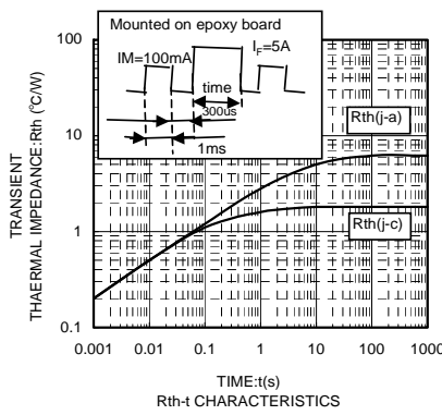
R_{th}-t CHARACTERISTICS
