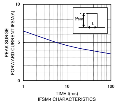
IFSM-t CHARACTERISTICS
