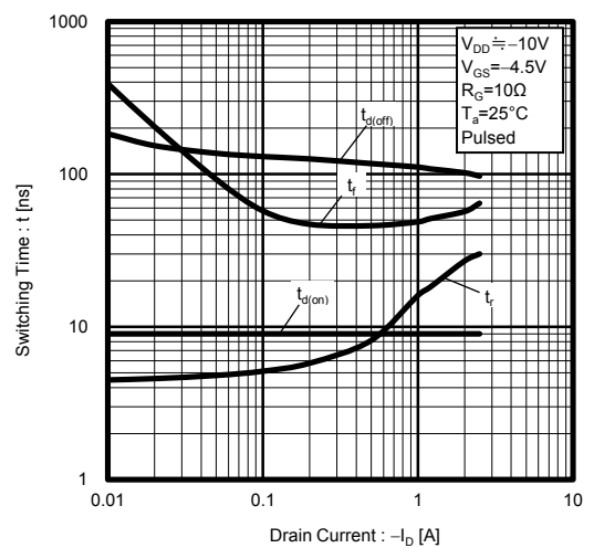
Fig.12 Switching Characteristics
