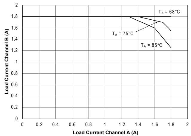
(a) V_{IN}=3.3\text{V} , V_{OUT}=2.5\text{V}
