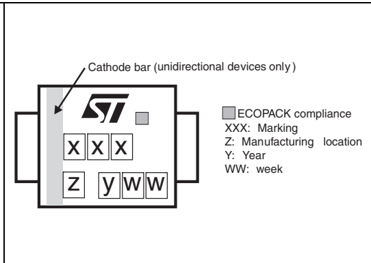
Figure 24. Marking layout (1)
