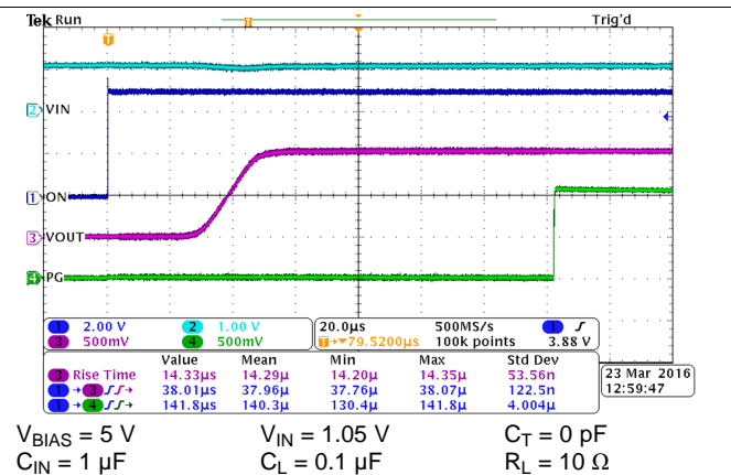
Figure 26. Turnon Response
