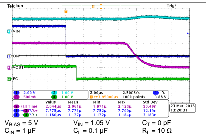
Figure 30. Turnon Response
