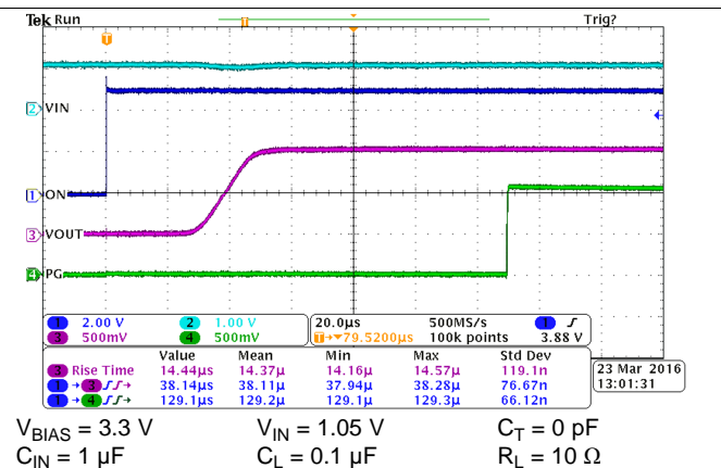
Figure 28. Turnon Response
