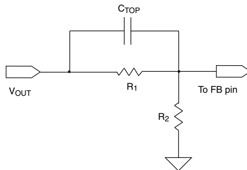
Fig. 13 - Capacitor Coupling to FB P IN
